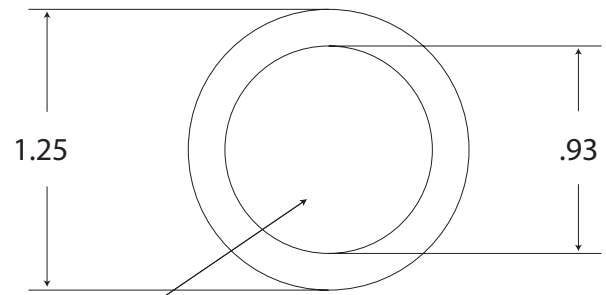
Sensing Surface
